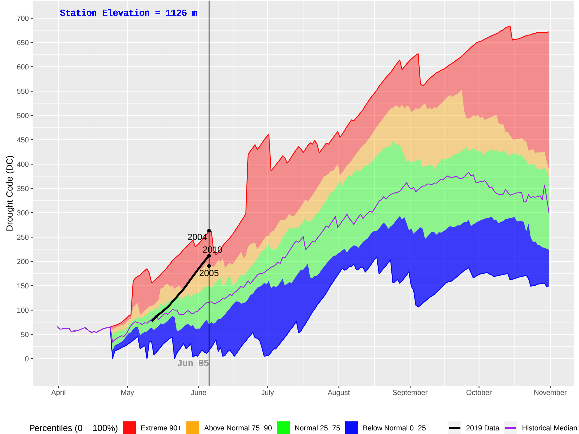
BLACKPINE (148) : Historical (1980–2018) and Current (2019) Daily Drought Code (DC)
