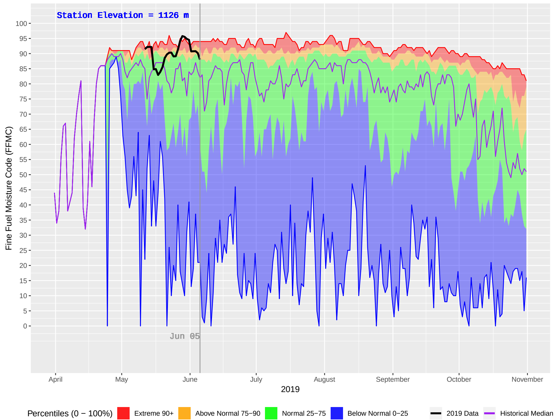
BLACKPINE (148) : Historical (1980–2018) and Current (2019) Daily Fine Fuel Moisture Code (FFMC)
