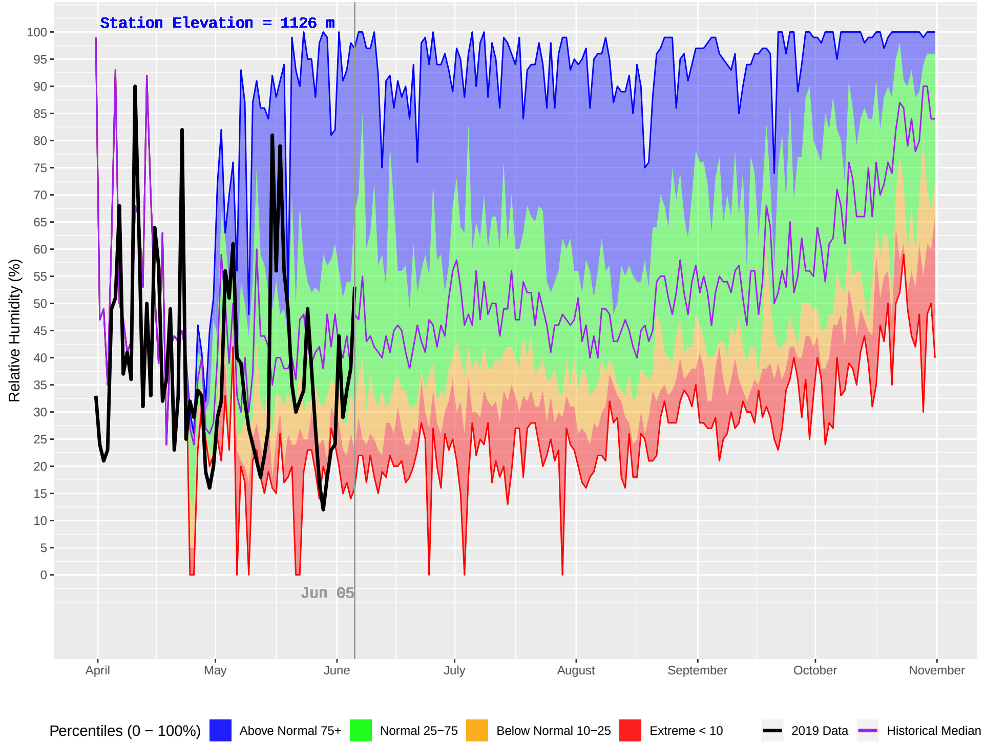
BLACKPINE (148) : Historical (1980–2018) and Current (2019) Daily Relative Humidity
