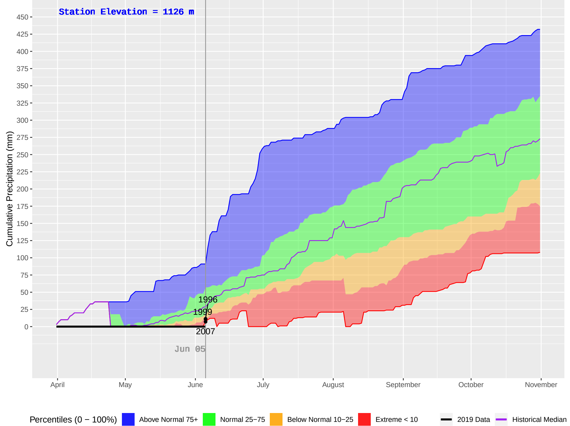
BLACKPINE (148) : Historical (1980–2018), Current (2019) Daily Cumulative Precipitation
