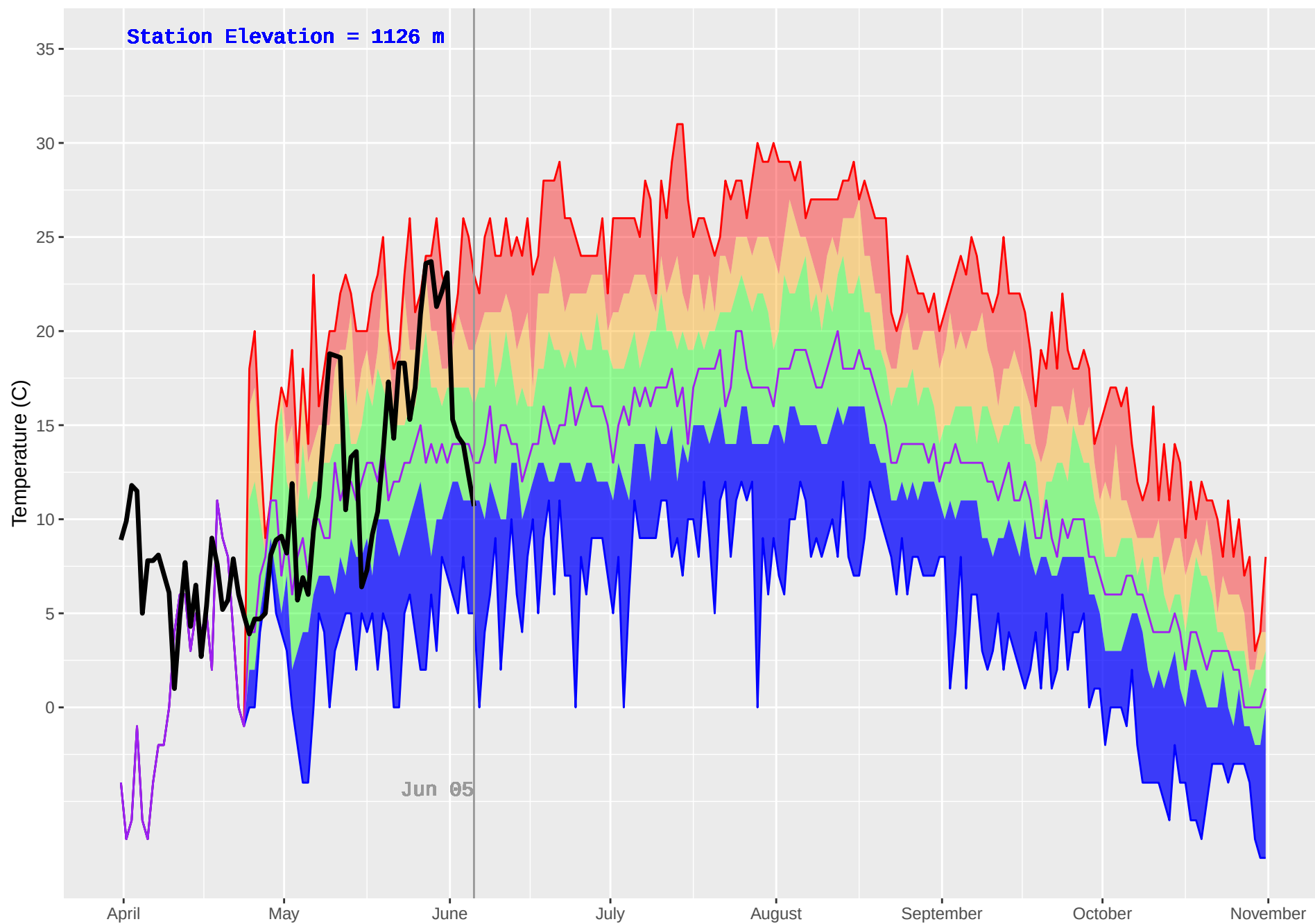
BLACKPINE (148) : Historical (1980–2018) and Current (2019) Daily Temperature
