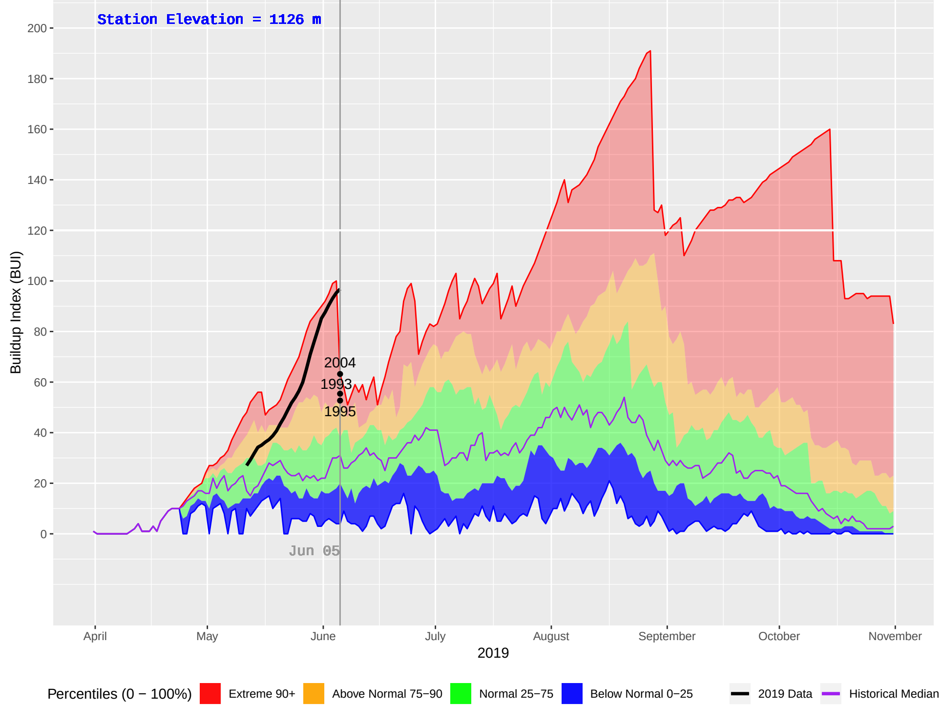
BLACKPINE (148) : Historical (1980–2018), Current (2019) Daily Buildup Index (BUI)
