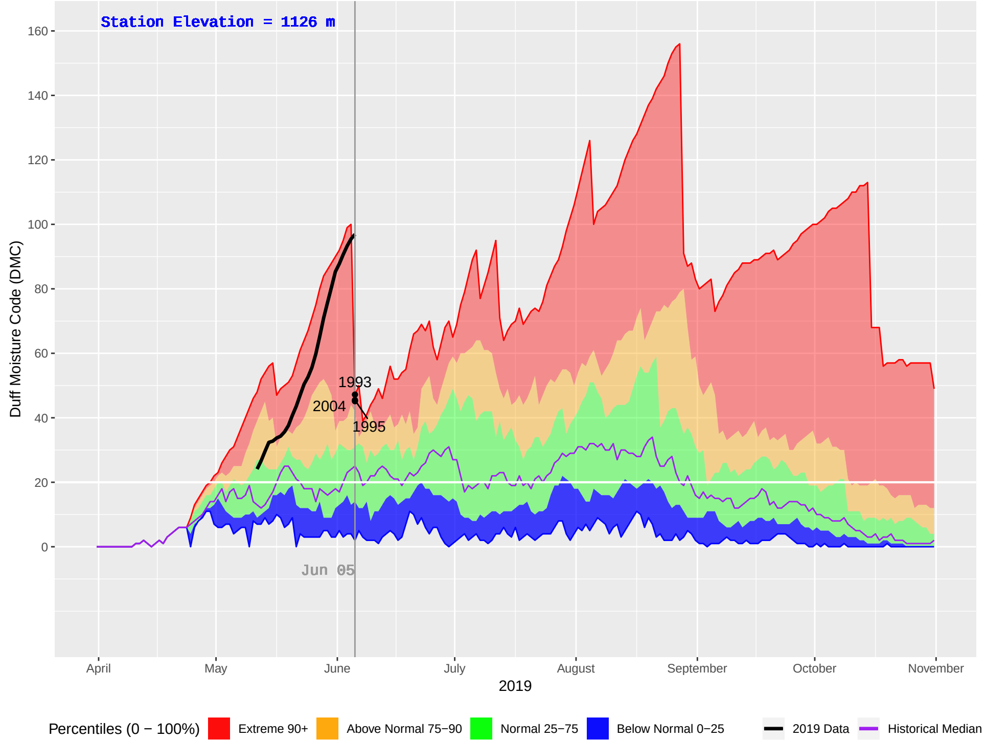
BLACKPINE (148) : Historical (1980–2018), Current (2019) Daily Duff Moisture Code (DMC)
